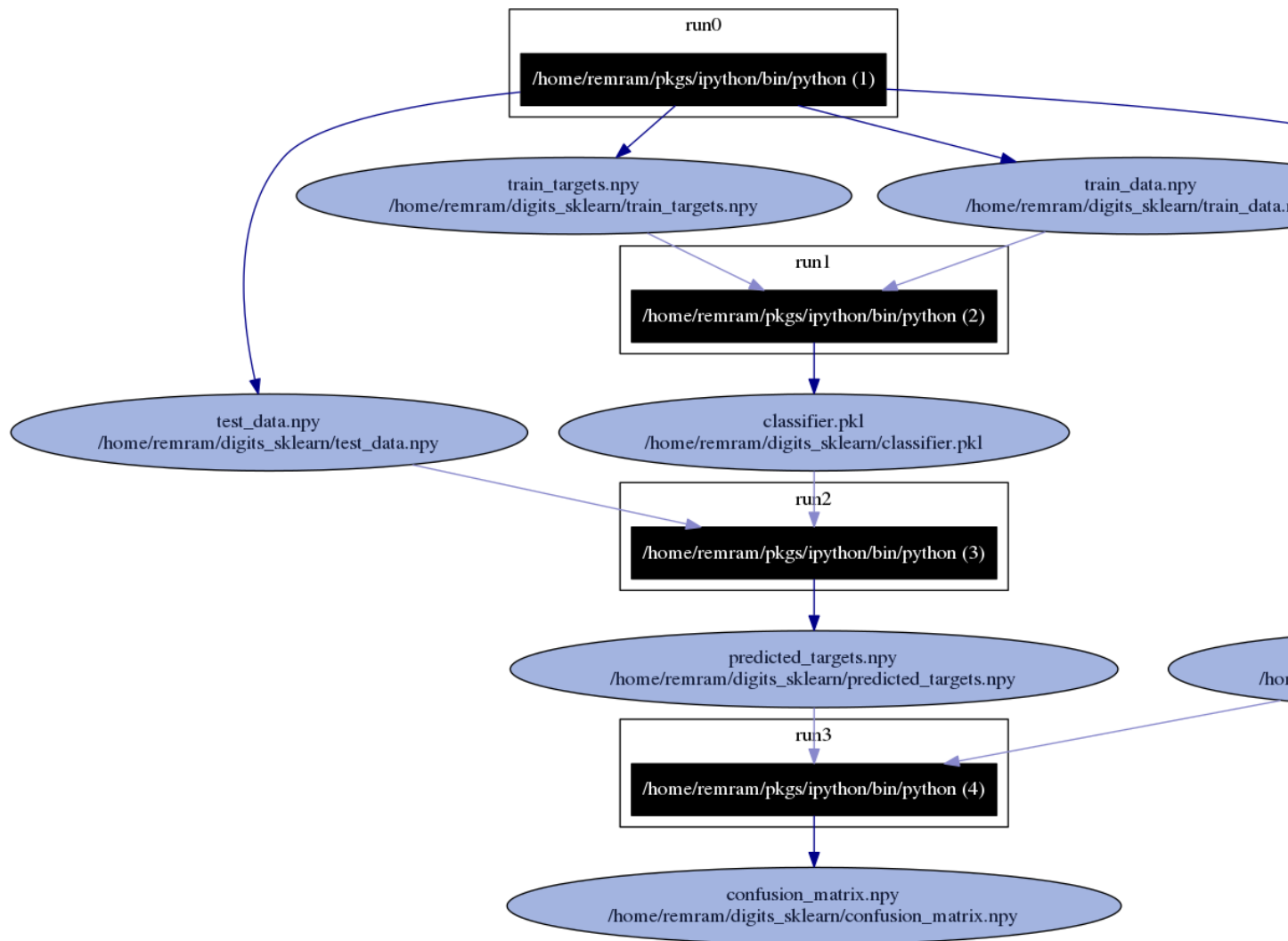
Fig. 1.2: Provenance graph showing input and output files for an experiment with 4 runs.
