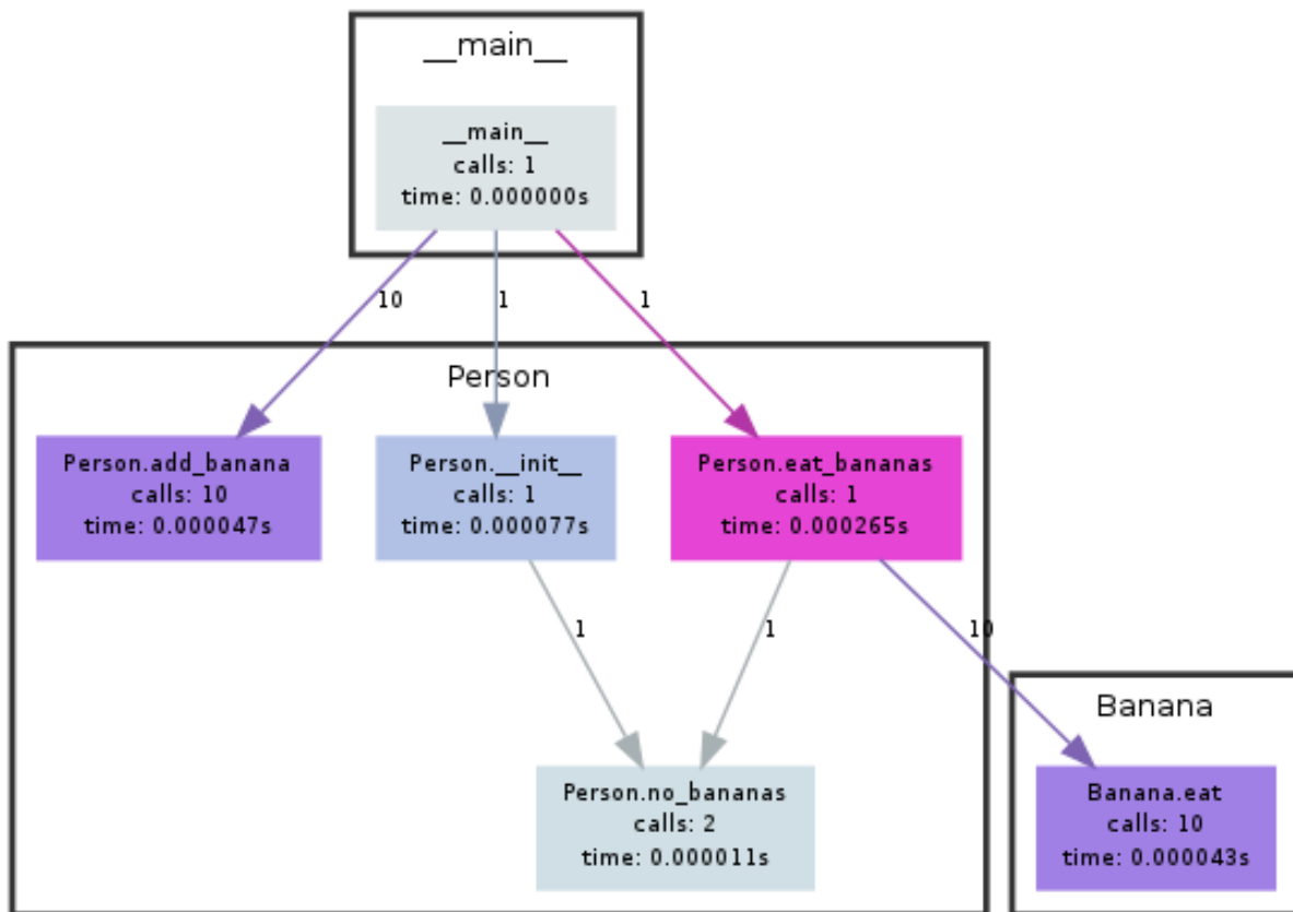
Generated by Python Call Graph v1.0.0 http://pycallgraph.slowchop.com
