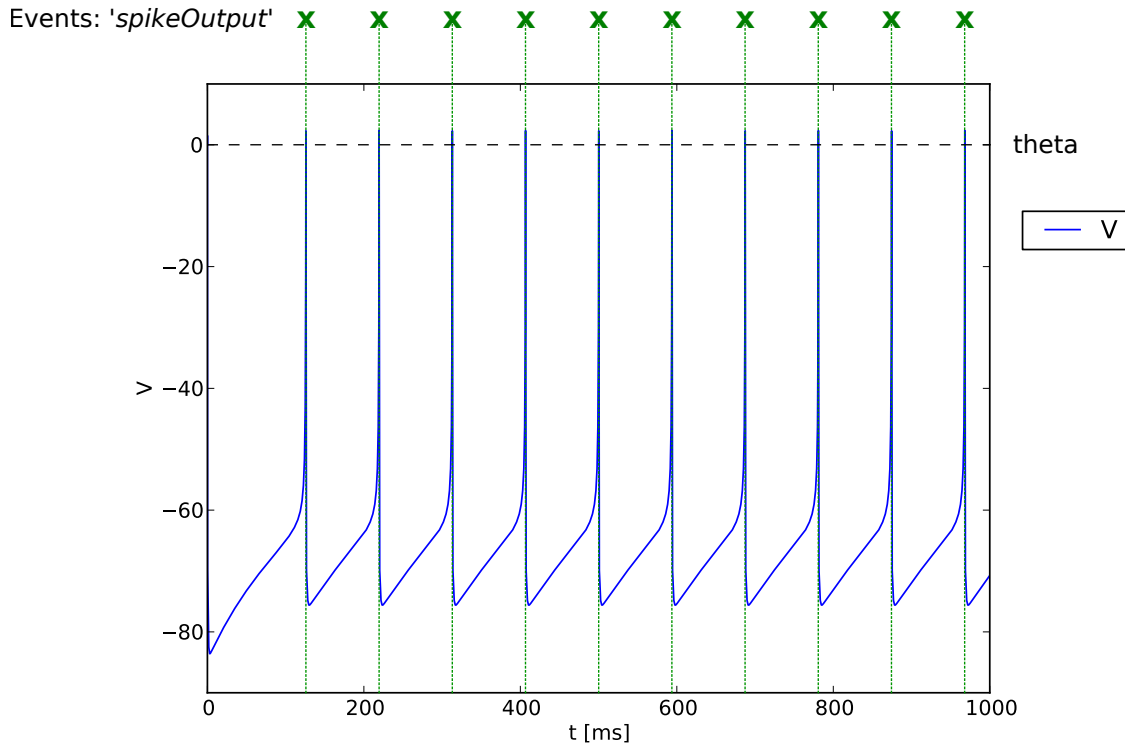
Fig. 2: Result of simulating of the XML model in this section
