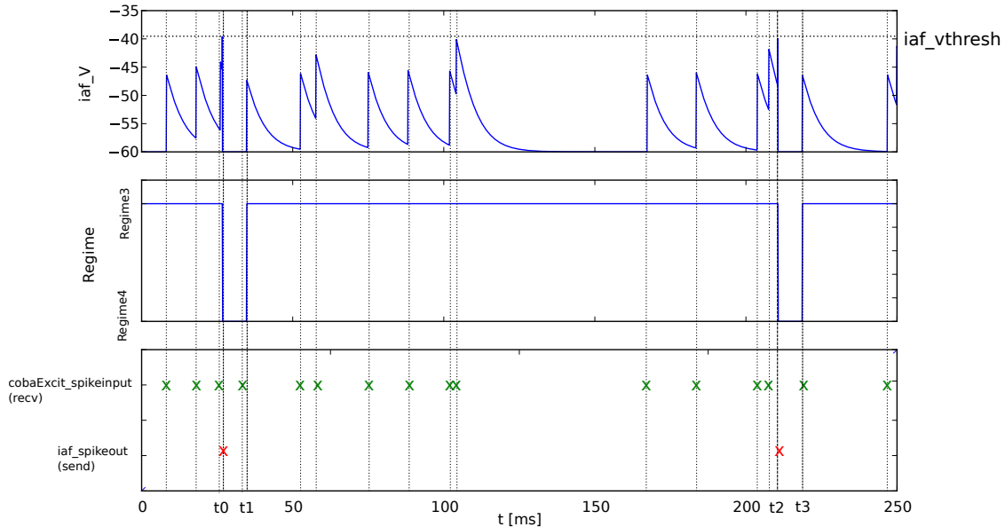
Fig. 4: Result of simulating of the XML model in this section. cobaExcit_spikeinput is fed events from an external Poisson generator in this simulation
