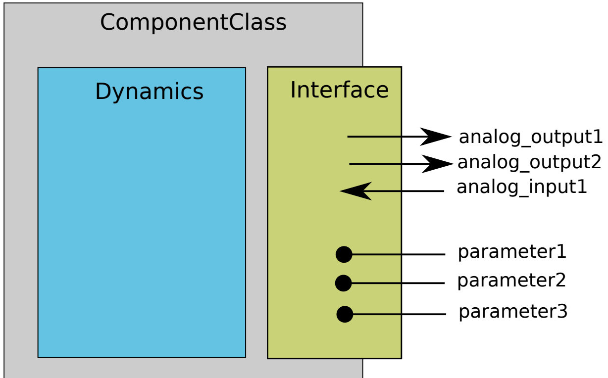
Fig. 1: ComponentClass Overview
