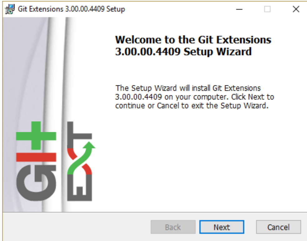
Fig. 1: Start installation.
