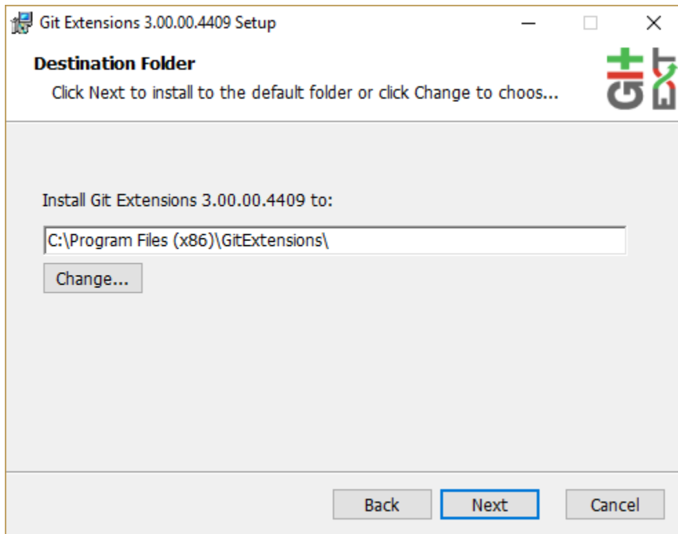
Fig. 3: Destination folder.
