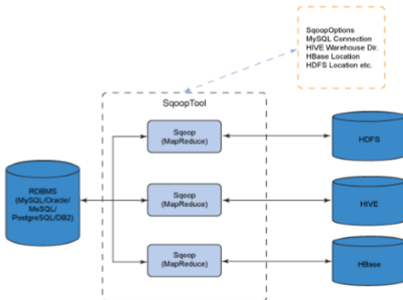
Figure 1: Sqoop data flow architecture
