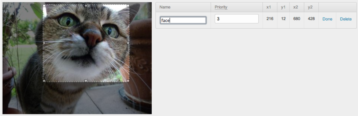
Fig. 1.2: The AreaWidget allows you to define areas of an image with click-and-drag. (Screenshot includes GrapPELLI.)
