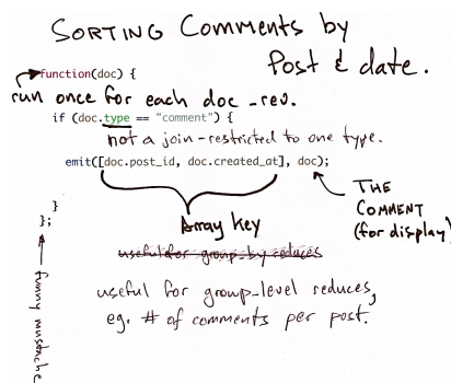
Fig. 1: Figure 1. Comments map function
