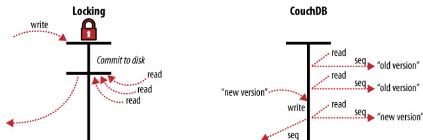
Fig. 6: Figure 3. MVCC means no locking
