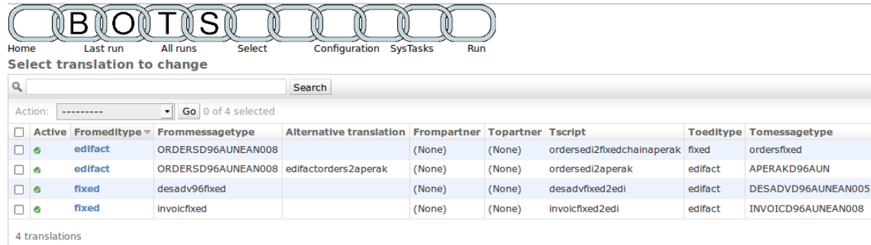
Fig. 7.1: Screenshot of configured translations-rules
